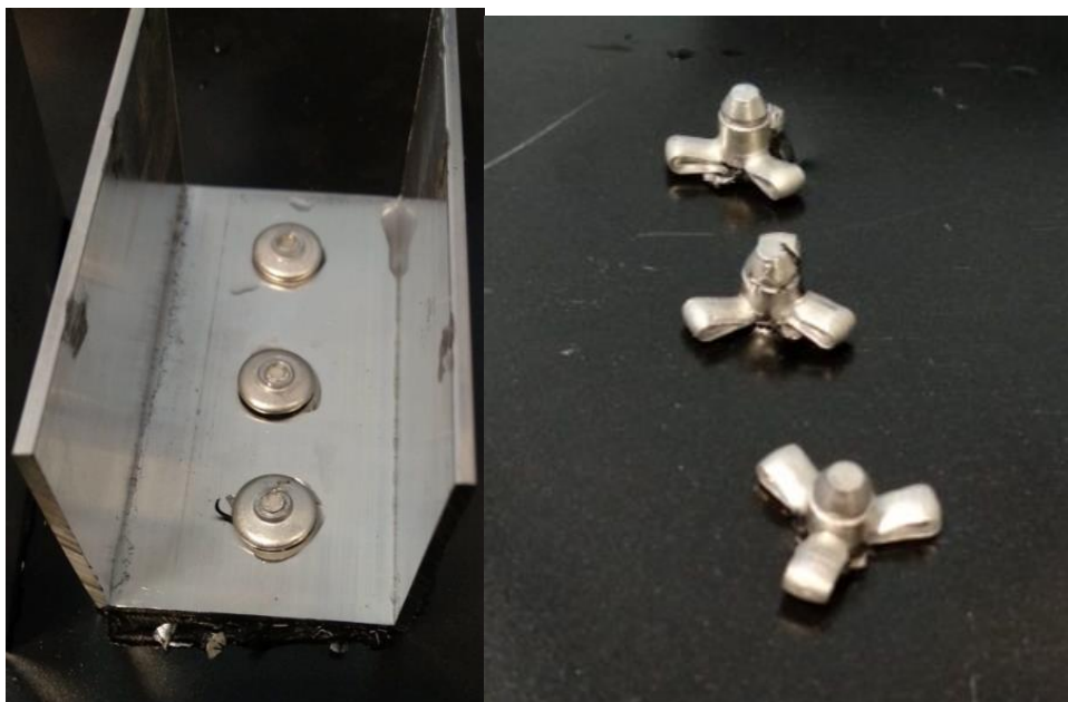
Application example 2: detail showing mounting on sheet metal to test watertightness
